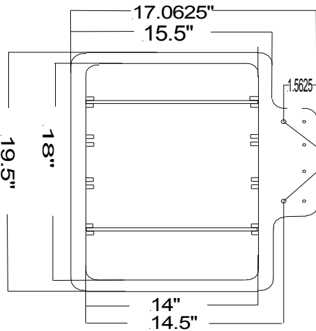
97 Series Plastic(Polystyrene) Recessed or Surface Mounted Cabinet
